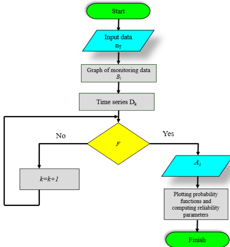
Fig. 2. 4 Flowchart for the statistical simulation modelling for reliability analysis
